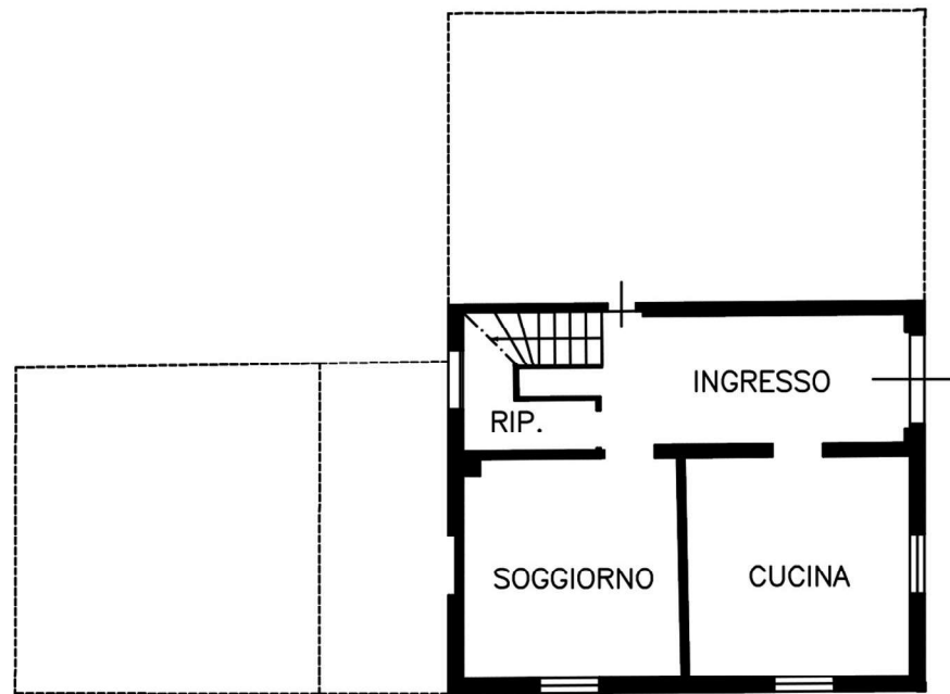
PIANO TERRA H=2.80
